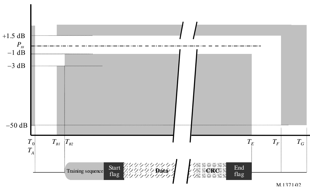
FIGURE 2 Transmitter output envelope versus time
