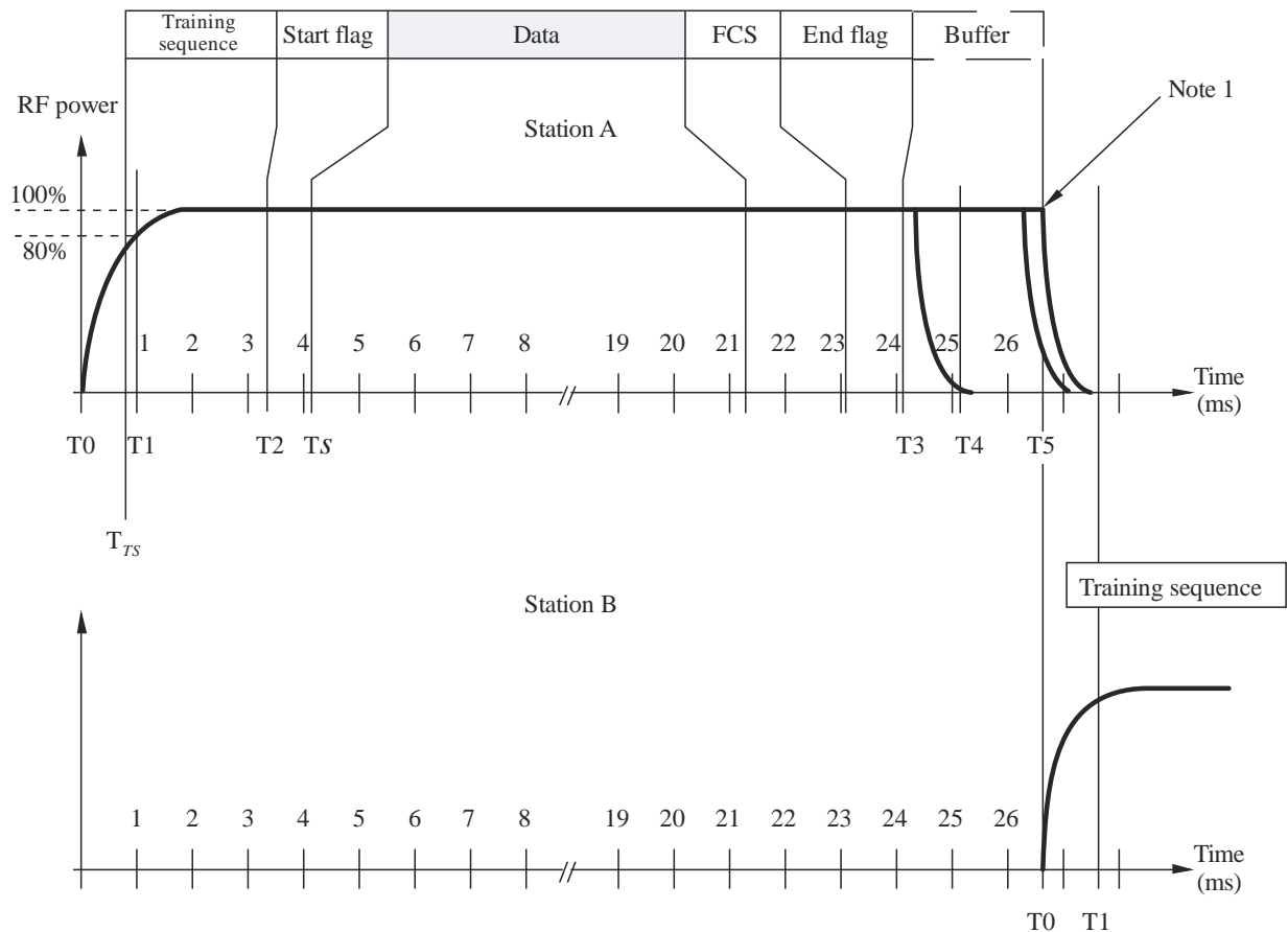
FIGURE 8 Transmission timing
